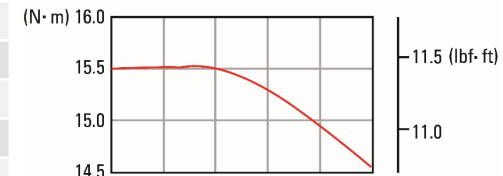
CRX275 SAE J1349 (NET)
